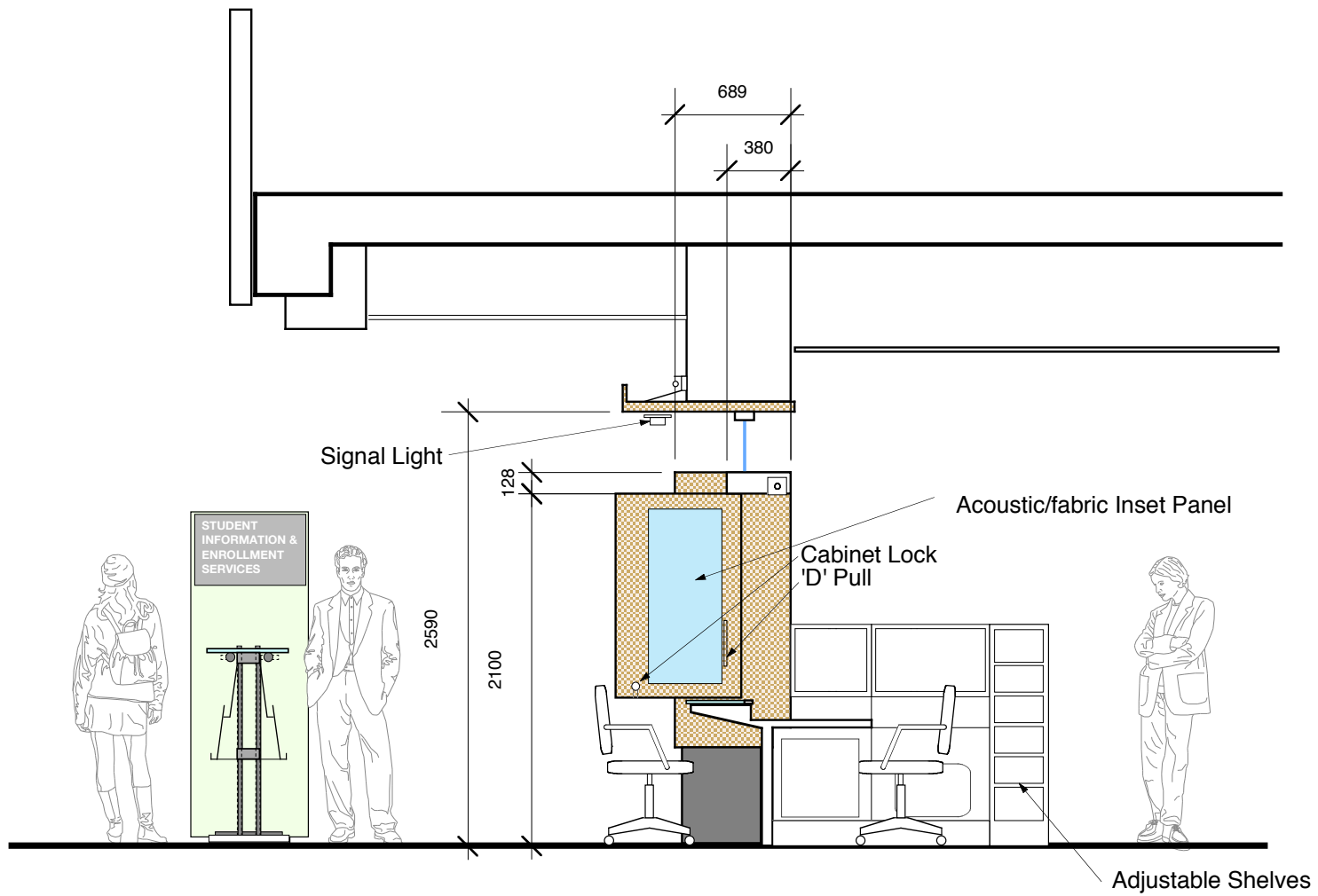
SIES COUNTERS - SECTION
